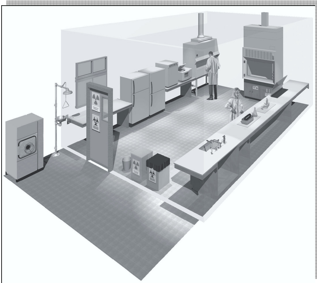
Schematic view, BSL 2 laboratory (source: Laboratory biosafety manual, WHO 2004).
